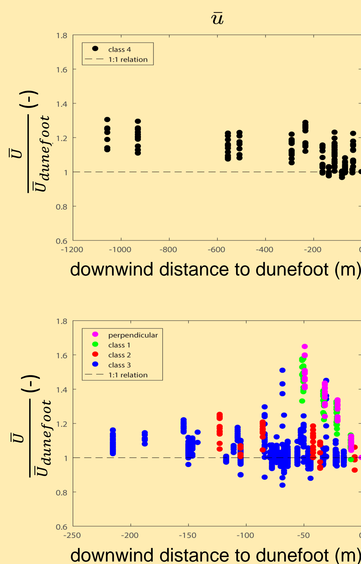
Fig 3: Relative mean wind speed as function of downwind distance to dunefoot for alongshore (upper) and oblique onshore winds (lower).
