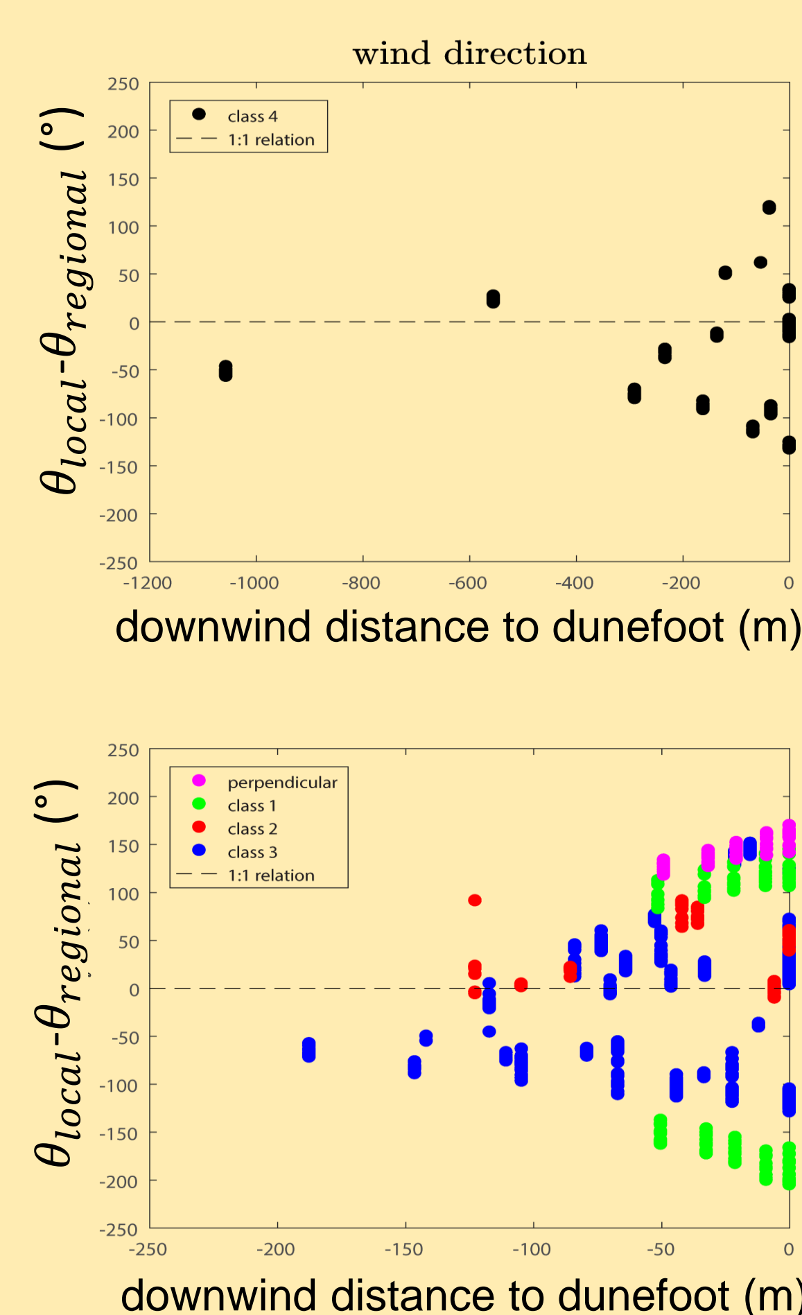
Fig 4: Steering of the regional wind as function of downwind distance to dunefoot for alongshore (upper) and oblique onshore winds (lower).
