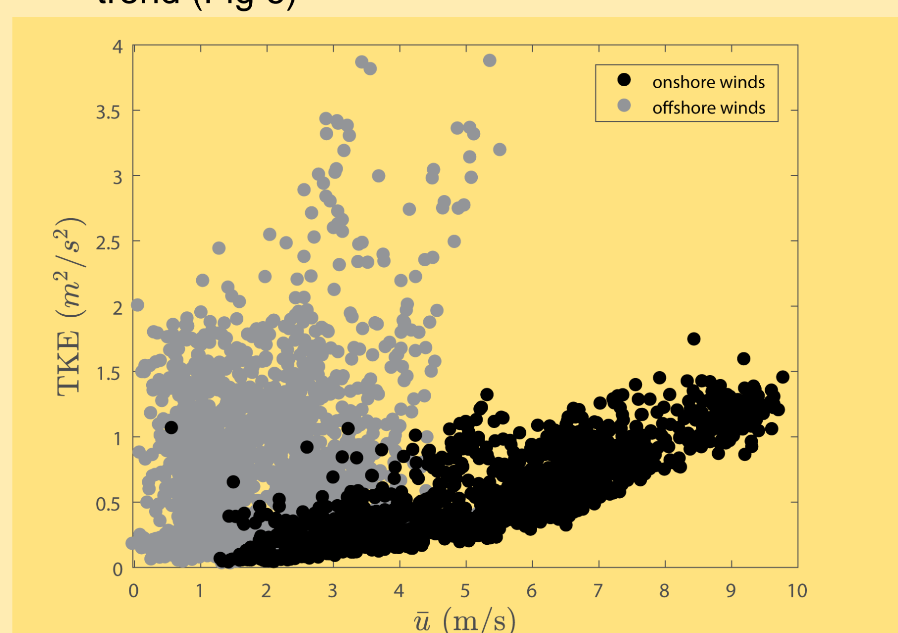
Fig 5: TKE as function of velocity
