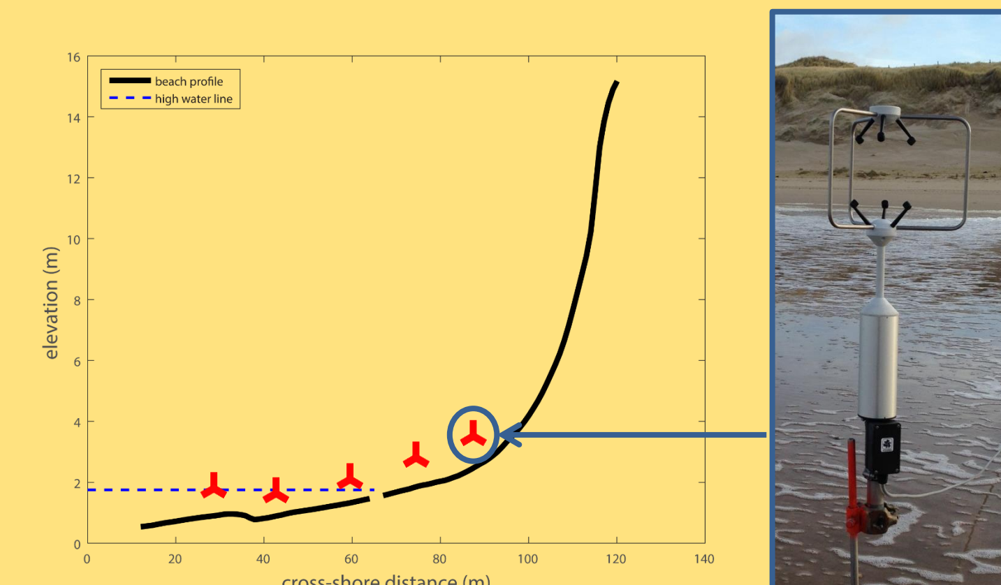
Fig 1: Field setup. Cross-shore array (left) with 4-6 ultrasonic anemometers (right).
