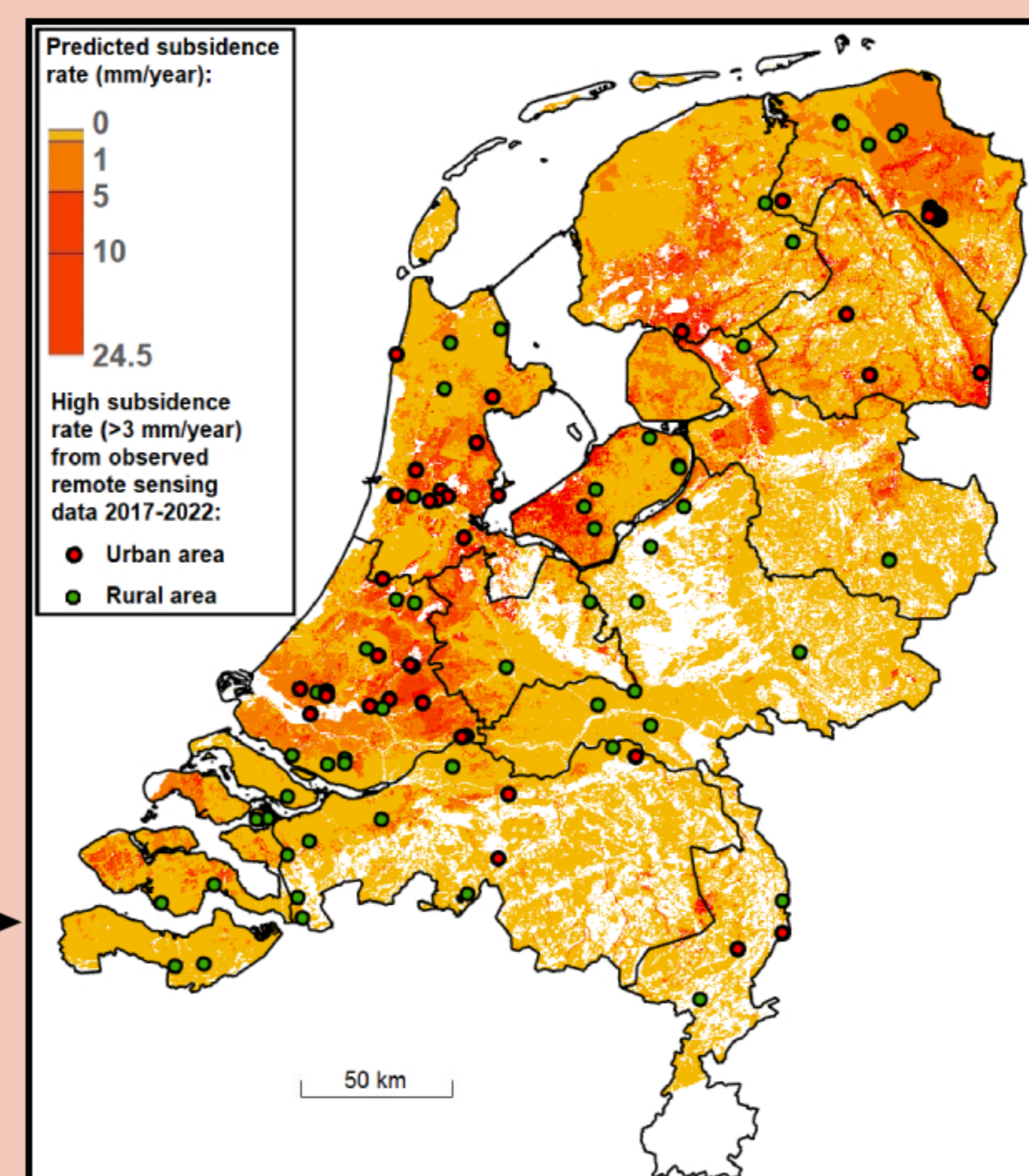
Fig.3: Predicted subsidence rate map of Atlantis 2050 for the low climate change scenario.
