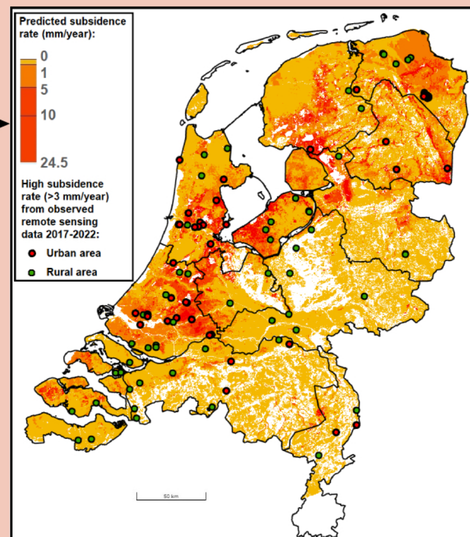
Fig.4: Predicted subsidence rate map of Atlantis 2050 for the high climate change scenario.
